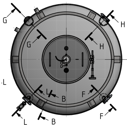
View J ( 1 : 10 )
