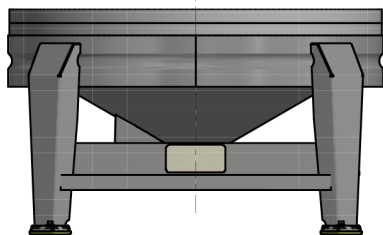
View D ( 1 : 10 )
