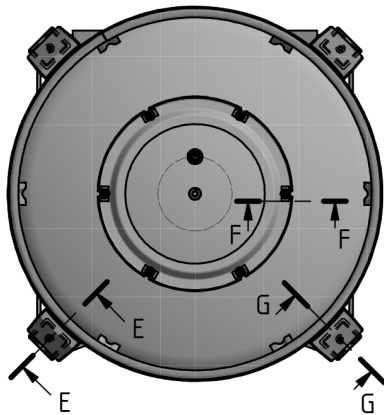
View D ( 1 : 10 )
